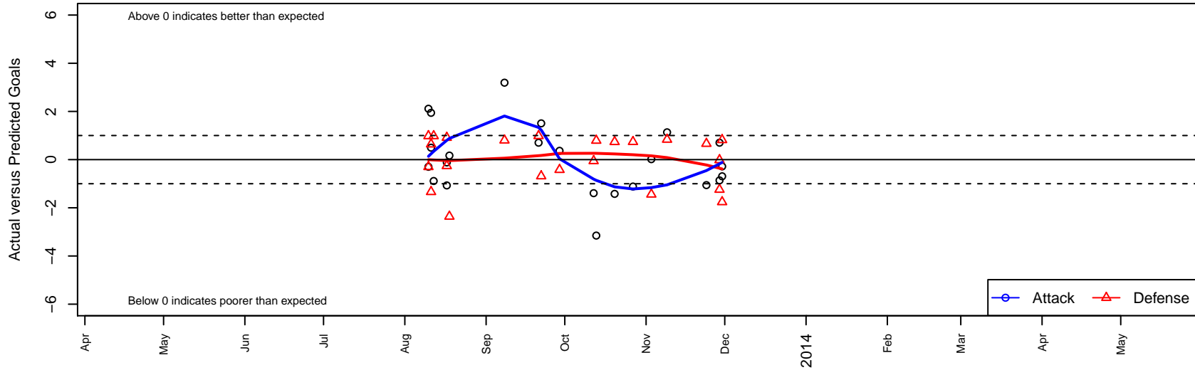
Real So Cal White B96 Dots are actual minus expected GF (blue circles) and GA (red triangles). Blue line is smoothed change in attack strength. Red is smoothed change in defense strength.
